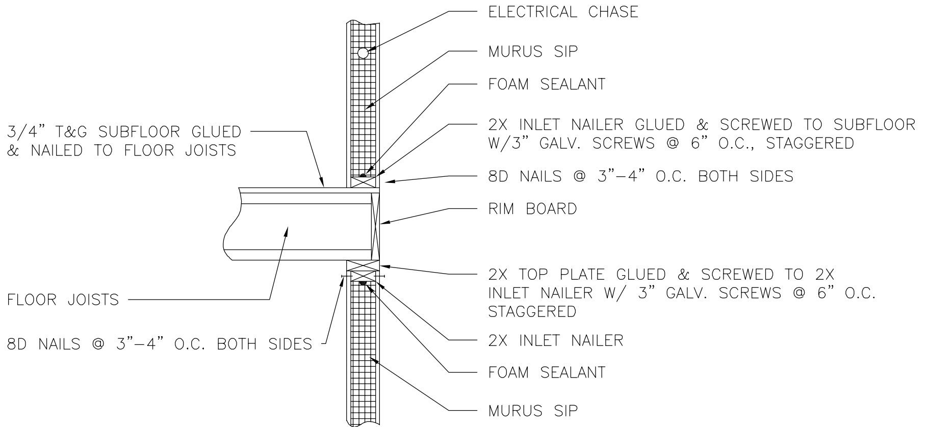
4 PLATFORM FRAMED @ UPPER FLOORS THE MURUS COMPANY
